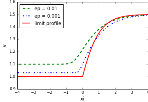
Figure 1: Asymptotic behavior of the profiles \mathbf{v}_\varepsilon with v_-^\varepsilon = 1 + \varepsilon^{1/\gamma} , v_+ = 1.5 and \gamma = 2 . The shift is fixed by prescribing \mathbf{v}_\varepsilon(0) = 1 + \varepsilon^{\frac{1}{\gamma+1}} .
